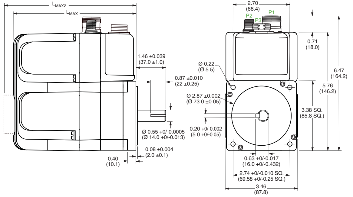
MDrive AccuStep lengths Inches (mm)
