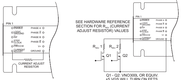
Fixed Value Current Adjust Resistor
