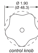
control knob
